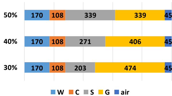
Figure. 1 Mix proportion of concrete
