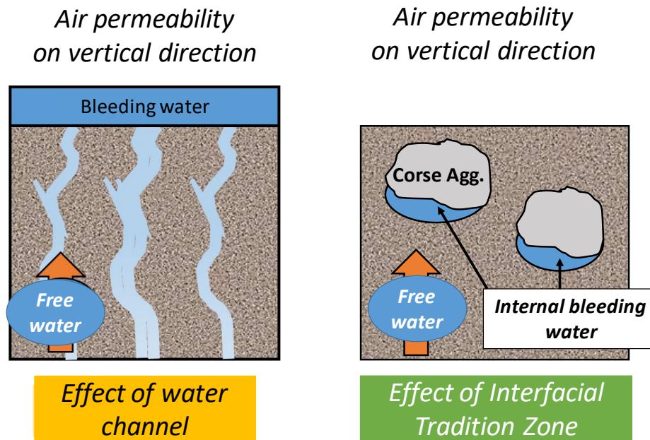
Figure. 6 Image of occurring gaps mechanism on different causes (Left: effect of water channel right: effect of bleeding for ITZ)
