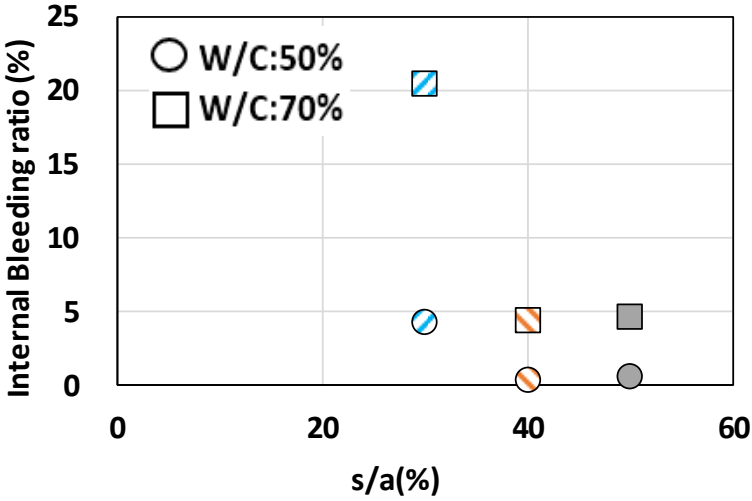
Figure. 5 Internal bleeding water ratio for different s/a values
