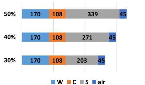
Figure. 2 Mix proportion of mortar
