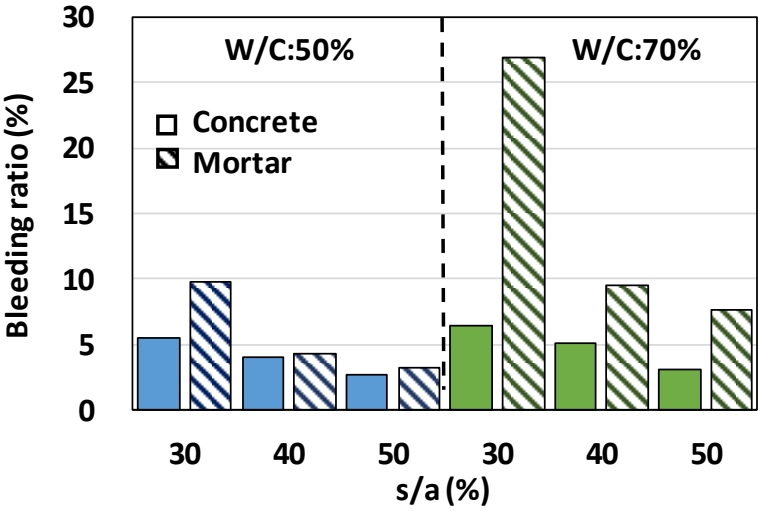
Figure. 4 Results of the bleeding test
