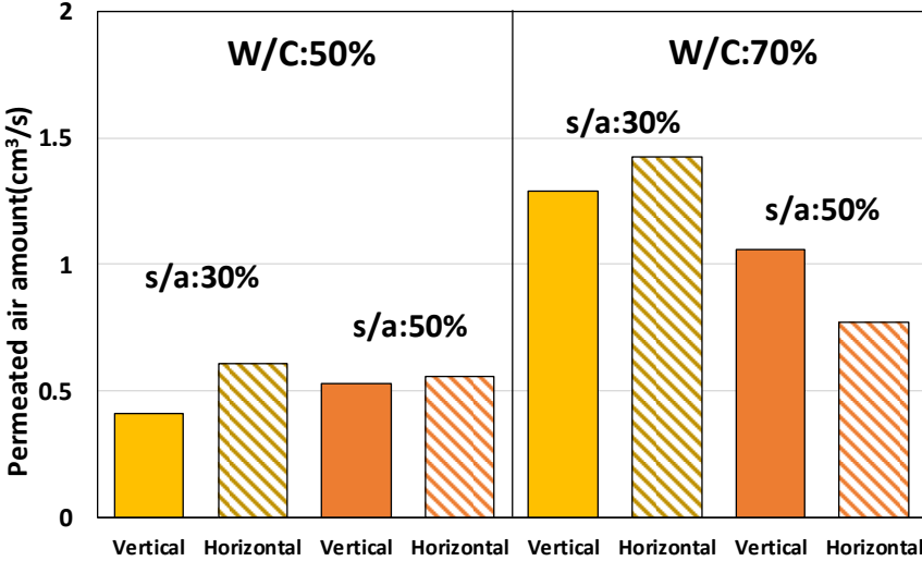
Figure. 7 Amount of permeated air
