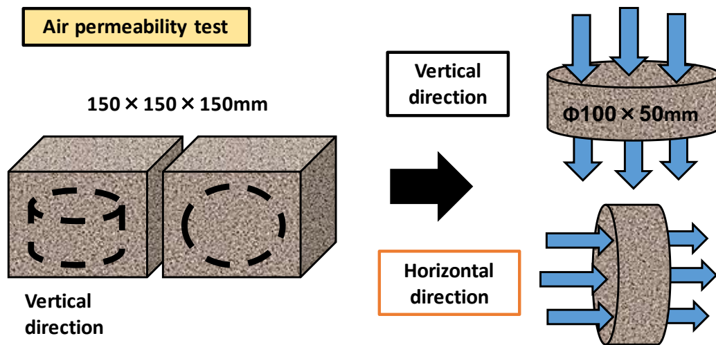
Figure. 3 Test flowchart
